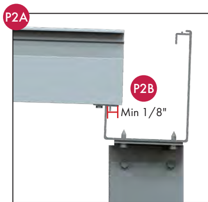
Gutter attachment
